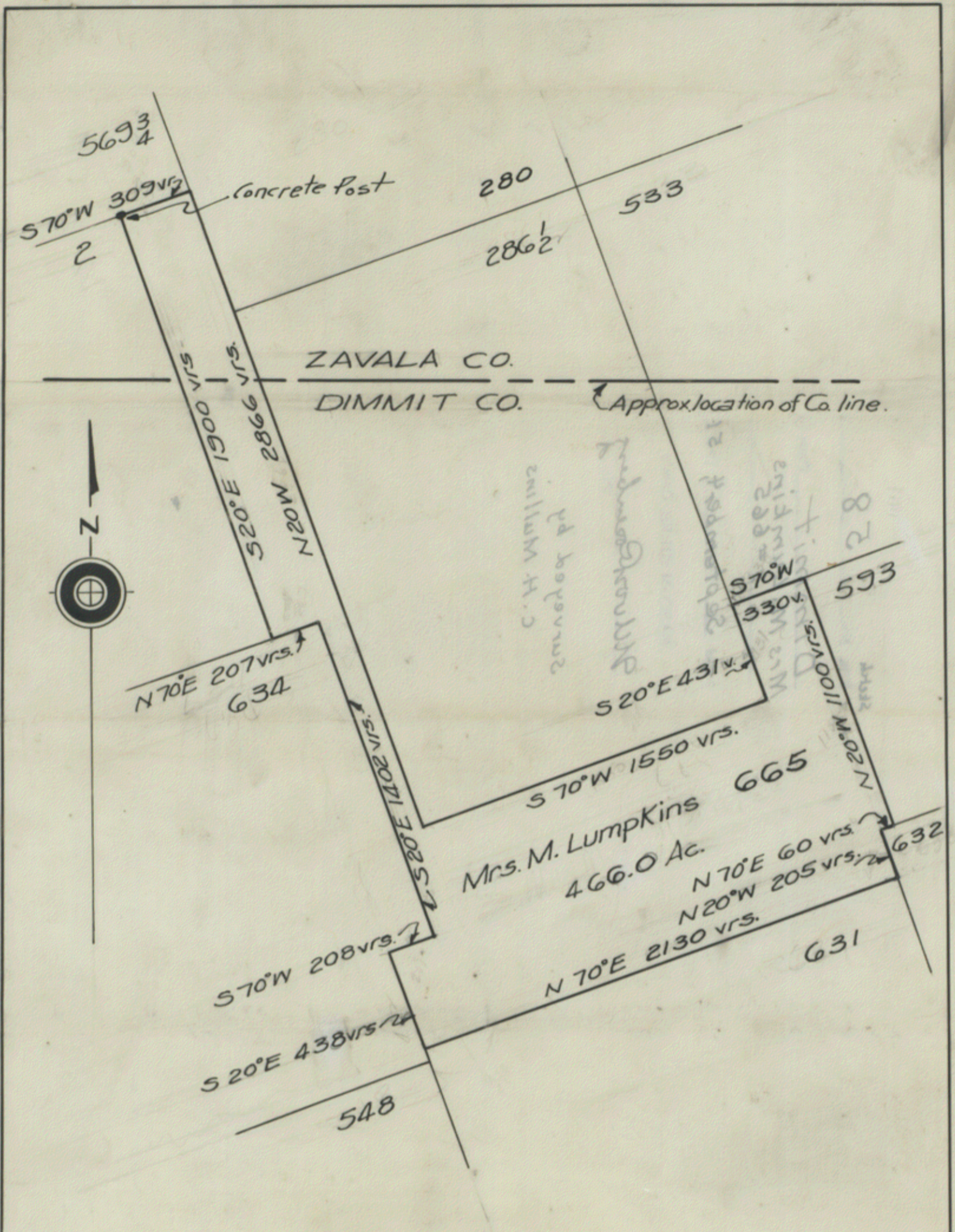
Plat Showing SURVEY NO. 665, MRS. M. LUMPKINS, IN DIMMIT AND ZAVALA COUNTYS. Made for J.M. Haigler by C.H. Mullins, April 26, 1951. Scale: 1" = 500 vrs.
